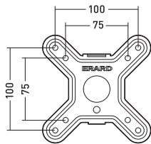
Platine TV
