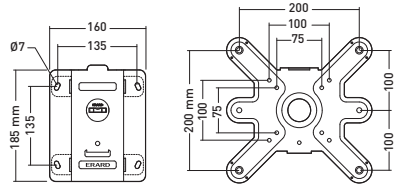
Platine murale
