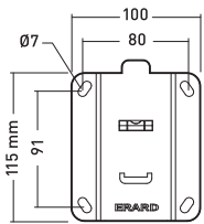
Platine murale
